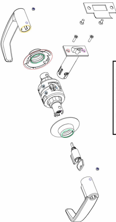
TZONE 11 LINE SERIES BORED IN LOCK
